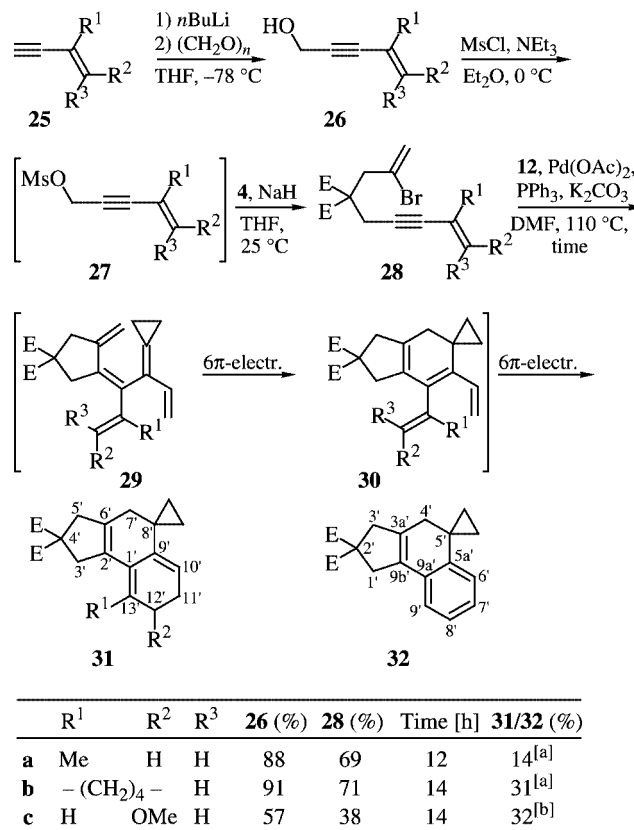
Scheme 8. Syntheses and domino-Heck co-cyclizations of 2-bromo-1,8-dien-6-ynes and bicyclopropylidene ( 12 ) by subsequent “transmissive electrocyclizations”. E = CO 2 Me.
