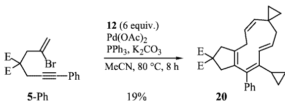
Scheme 5. Formation of the 11-membered ring compound 20 from 5-Ph and 12 . E = \text{CO}_2\text{Me} .
