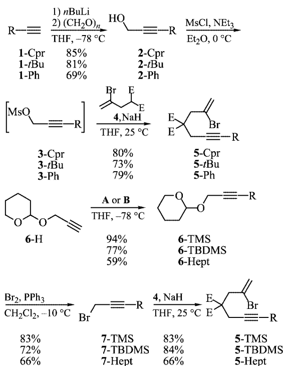
Scheme 1. Preparation of acyclic 2-bromo-1,6-enynes. Reagents and conditions: A : n BuLi, Me 3 SiCl or t BuMe 2 SiCl, THF, -78 °C; B : n BuLi, 6-heptenyl bromide, HMPA, THF, -78 °C. E = CO 2 Me; R = Cpr (cyclopropyl), t Bu, Ph and Hept (6'-heptenyl).
