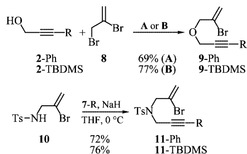
Scheme 2. Preparation of heteroatom-containing 2-bromo-1,6-enynes. Reagents and conditions: A : CETAB (cetyltrimethylammonium bromide), NaOH, CH 2 Cl 2 , H 2 O, 25 °C; B : NaH, THF, 0 → 25 °C.
