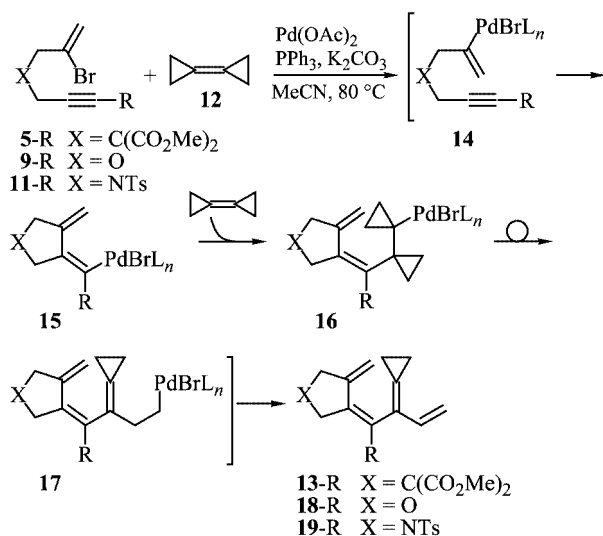
Scheme 4. Formation of cross-conjugated tetraenes from 2-bromo-1,6-enynes and bicyclopopylidene ( 12 ). For reaction details see Table 2.
