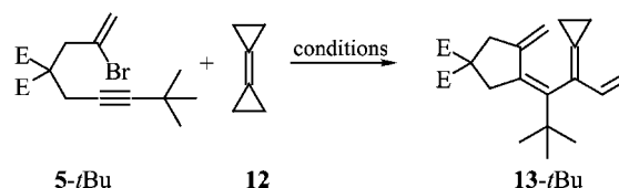
Scheme 3. E = CO 2 Me. For reaction details see Table 1.
