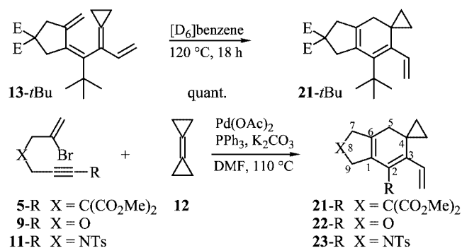
Scheme 6. Thermal 6\pi -electrocyclization of 13- t Bu and direct formation of such products from 5-R , 9-R , 11-R and bicyclopropylidene ( 12 ). E = \text{CO}_2\text{Me} . For reaction details see Table 3.
