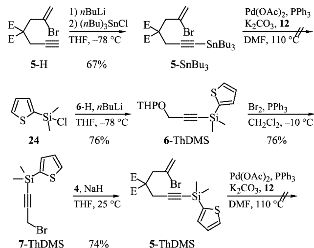
Scheme 7. Syntheses and attempted cyclizations of tributylstannyl- and (dimethylthiophenylsilyl)-substituted 2-bromo-1,6-enynes. E = CO 2 Me.
